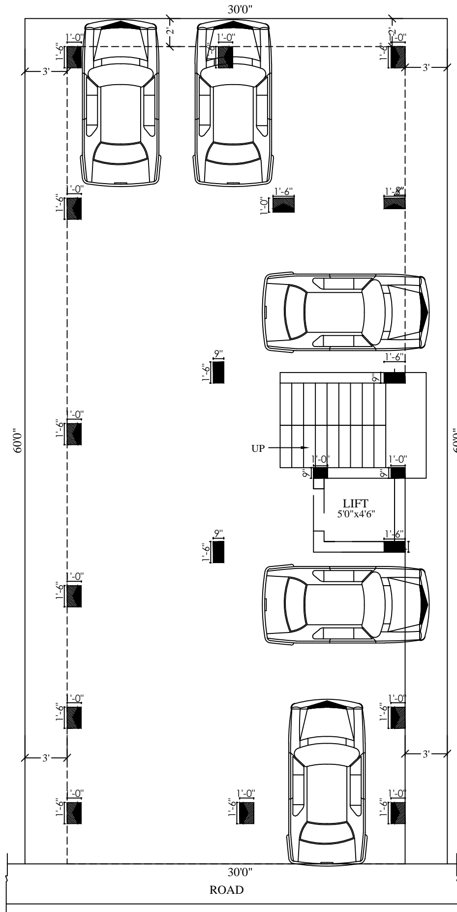
SITE CUM STILT FLOOR PLAN
