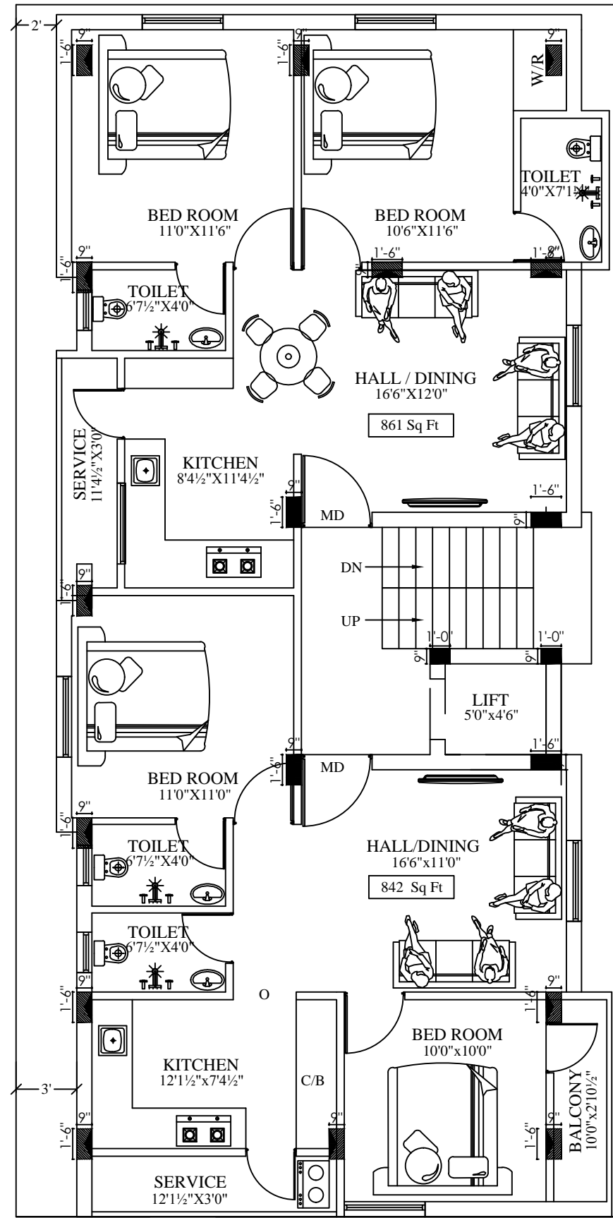
FIRST & SECOND FLOOR PLAN
